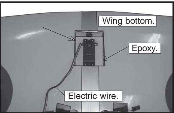
INSTALLING RETRACTABLE LANDING GEAR.
